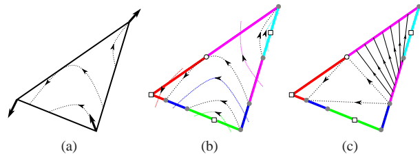
Figure 3: Edge map for a triangle. (a) Within a triangle, the vector is represented by interpolating three vectors at its vertices. (b) Our representation subdivides the boundary into a set of intervals, which map inflow to outflow for a triangle. (c) Given an entry point to a triangle, its corresponding exit point can be obtained by approximating the map linearly, thus replacing streamline integration with a step across the triangle.
