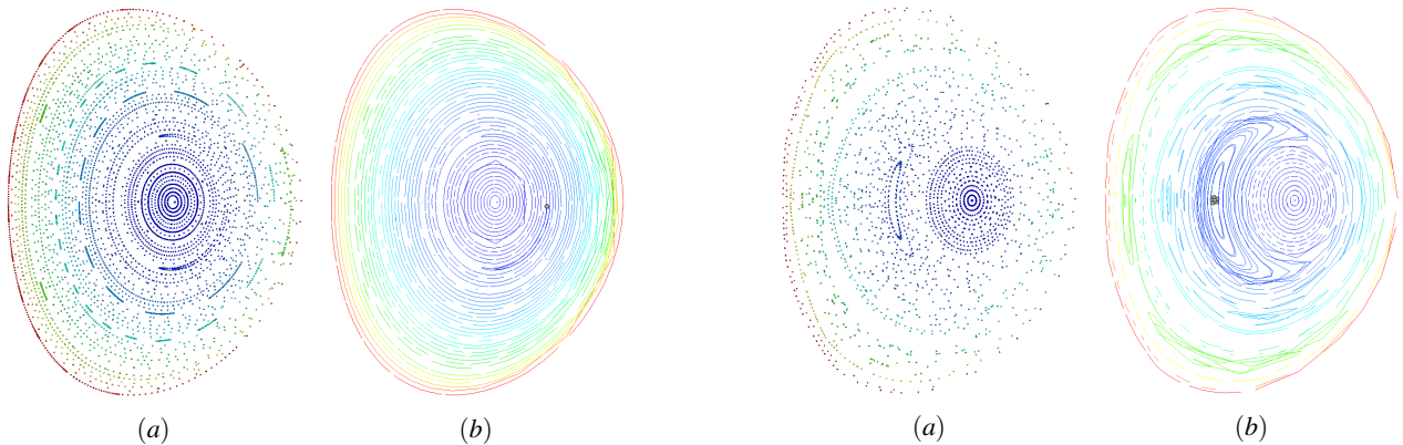
Fig. 16. (a) A Poincaré plot of 51 fieldlines. Each fieldline generates 300 puncture points. (b) The same plot using a near minimal number of puncture points that have been connected. There are two thin island chains (one green and one blue) that are partially visible without connectivity.
